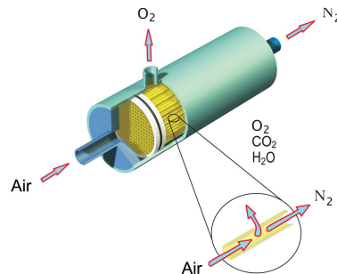
Membrane gas separation - Wikipedia.
