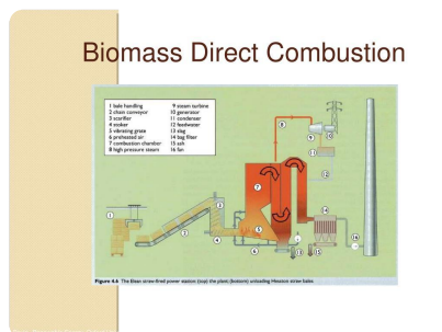
biomass direct combustion.
